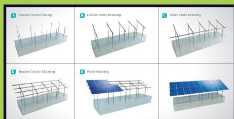
Steel Ground Mounting System with 2 Vertical Panels
