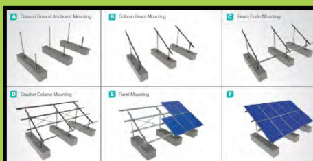
Steel Mounting System Anchored on Concrete Base with 2 Vertical Panels
